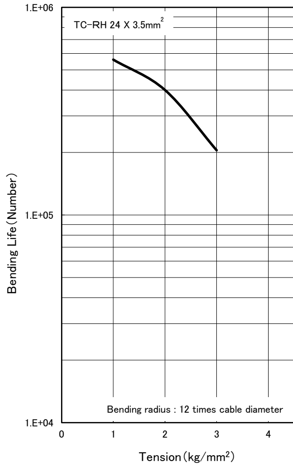
Fig.3 Bending Life of TC-RH (Tension vs Bending Life)
