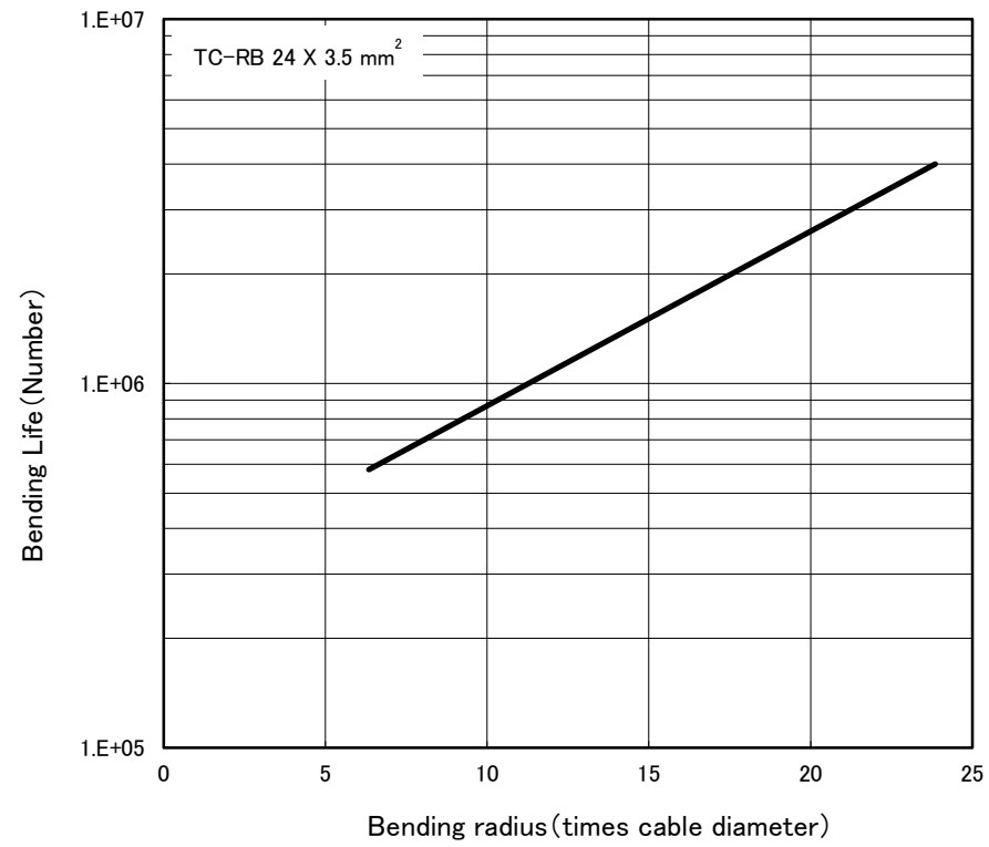
Fig.5 Bending Life of TC-RB (Bending Radius vs Bending Life)
