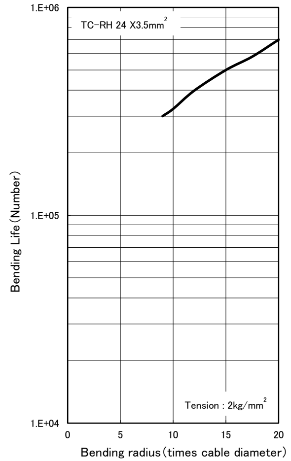
Fig.4 Bending Life of TC-RH (Bending Radius vs Bending Life)
