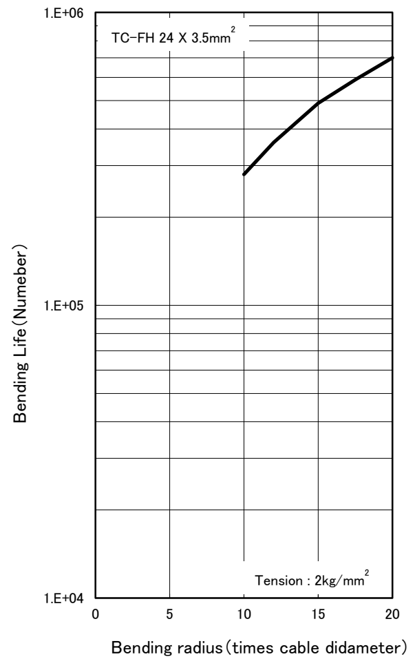
Fig.2 Bending Life of TC-FH (Bending Radius vs Bending Life)
