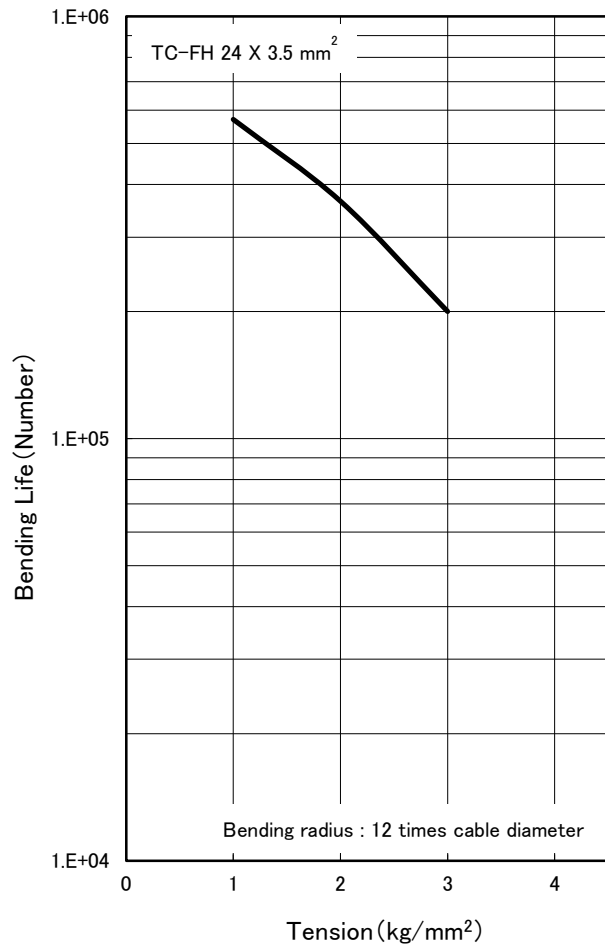
Fig.1 Bending Life of TC-FH (Tension vs Bending Life)
